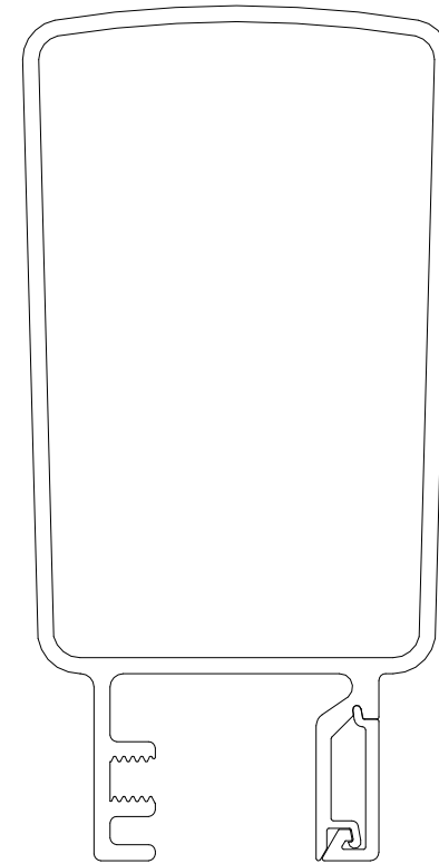
#902 TOP RAIL WITH #907 SCREW COVER
